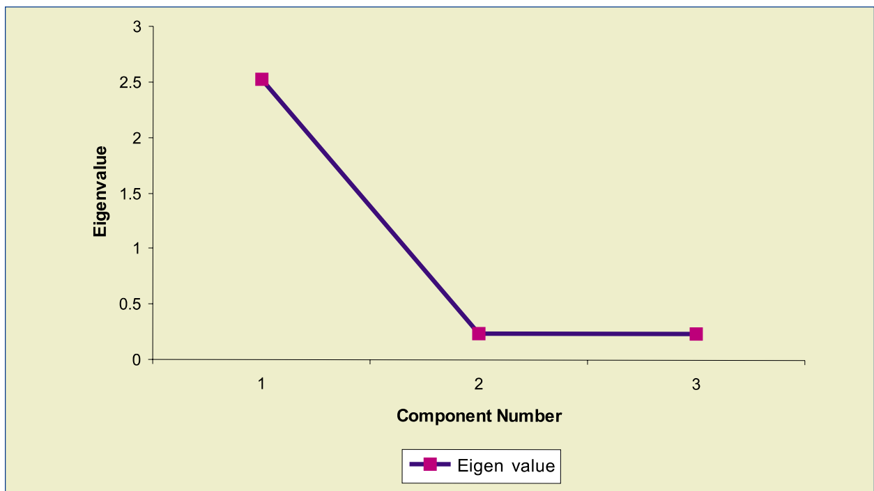
Figure 2.2: Scree Plot
